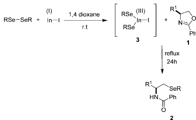
Scheme 1. Indium(I) iodide mediated oxazoline ring opening with diorganoyl diselenides.
