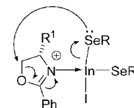
Figure 1. Proposed mechanism for the oxazoline ring-opening reaction.
