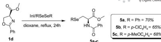
Scheme 3. Synthesis of selenocysteine derivatives.
