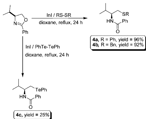
Scheme 2. Synthesis of chiral \beta -chalcogeno amides.
